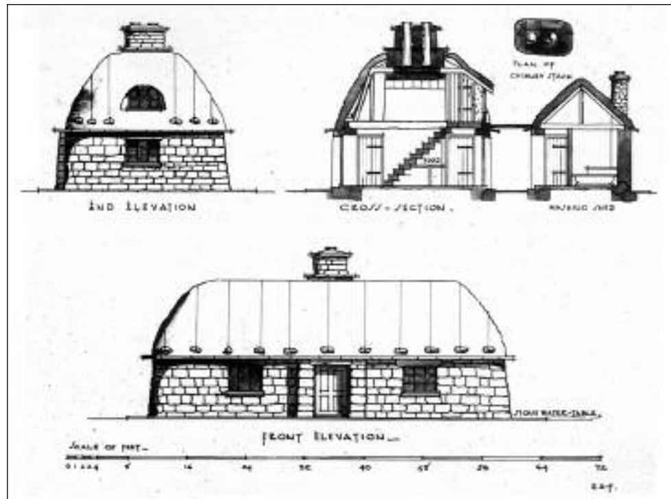
FIGURE 6. Werner Kissling, design for a two-story cottage based upon a traditional Highland blackhouse. Competition entry, Royal Institute of Architects in Scotland, 1930s. (Crown Copyright).
